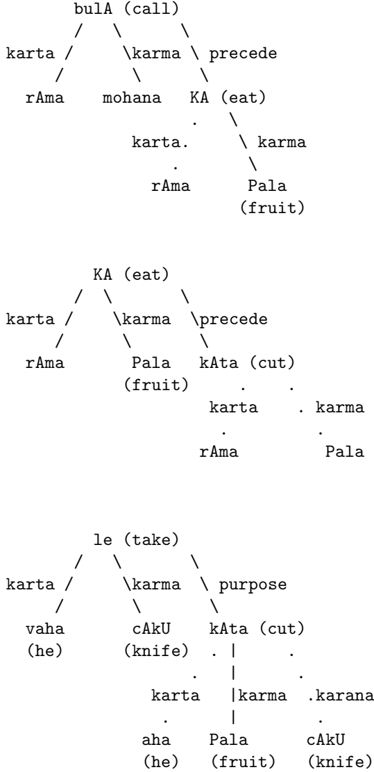
Fig. 6: Modifier-modified relations for sentences G.1, G.2 and G.3, respectively. (Shared karakas shown by dotted lines.)
