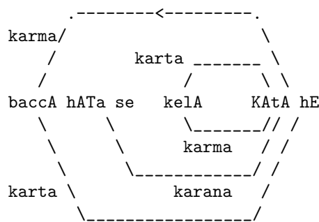
Fig. 4: Constraint graph
